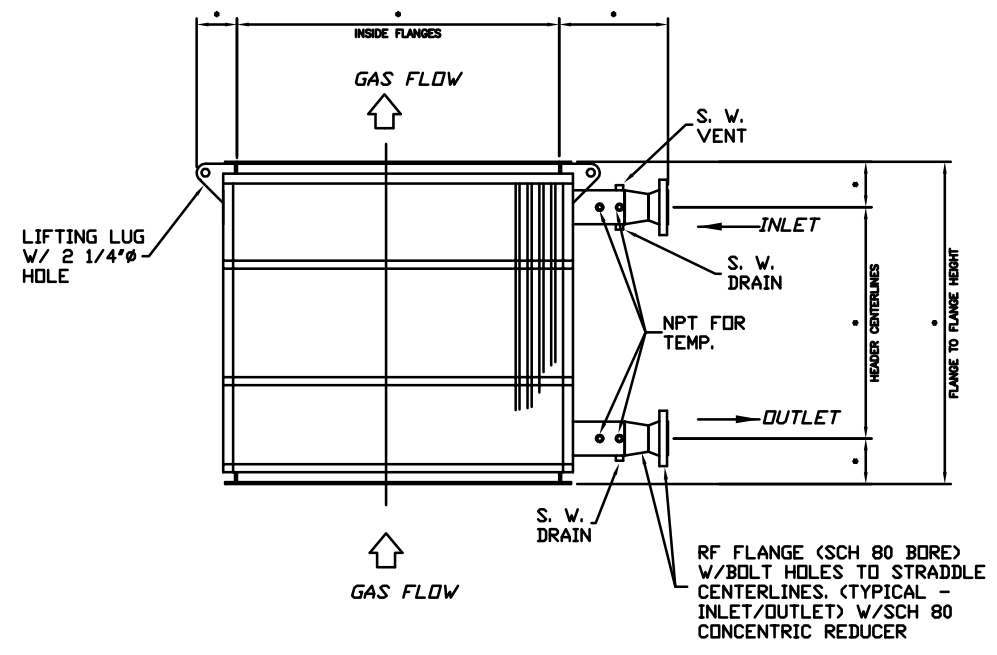
END VIEW
