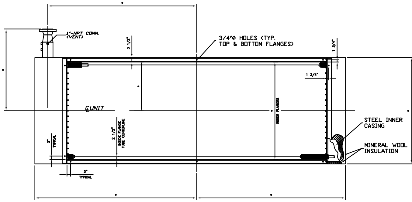
PLAN VIEW
