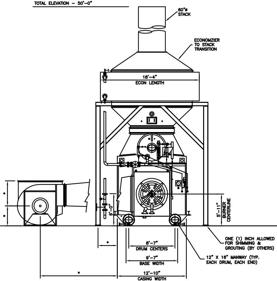
BURNER END VIEW
