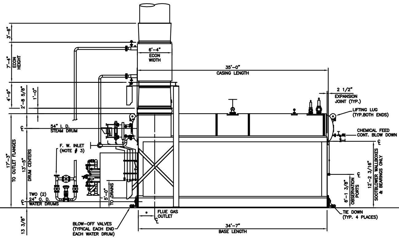
SIDE ELEVATION
